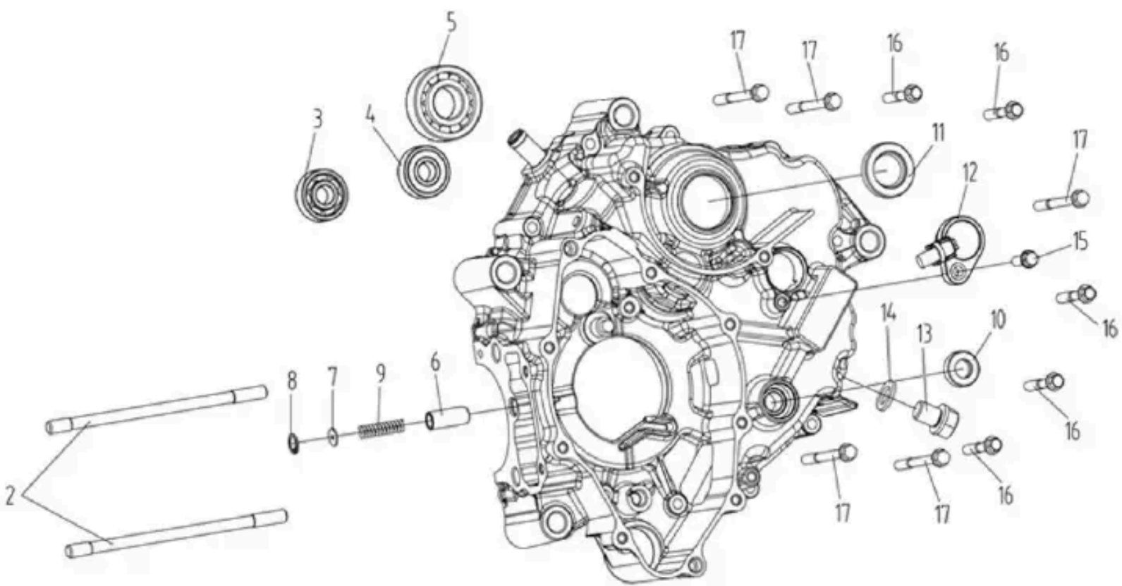
E01 CRANKCASE COMP.,LEFT
