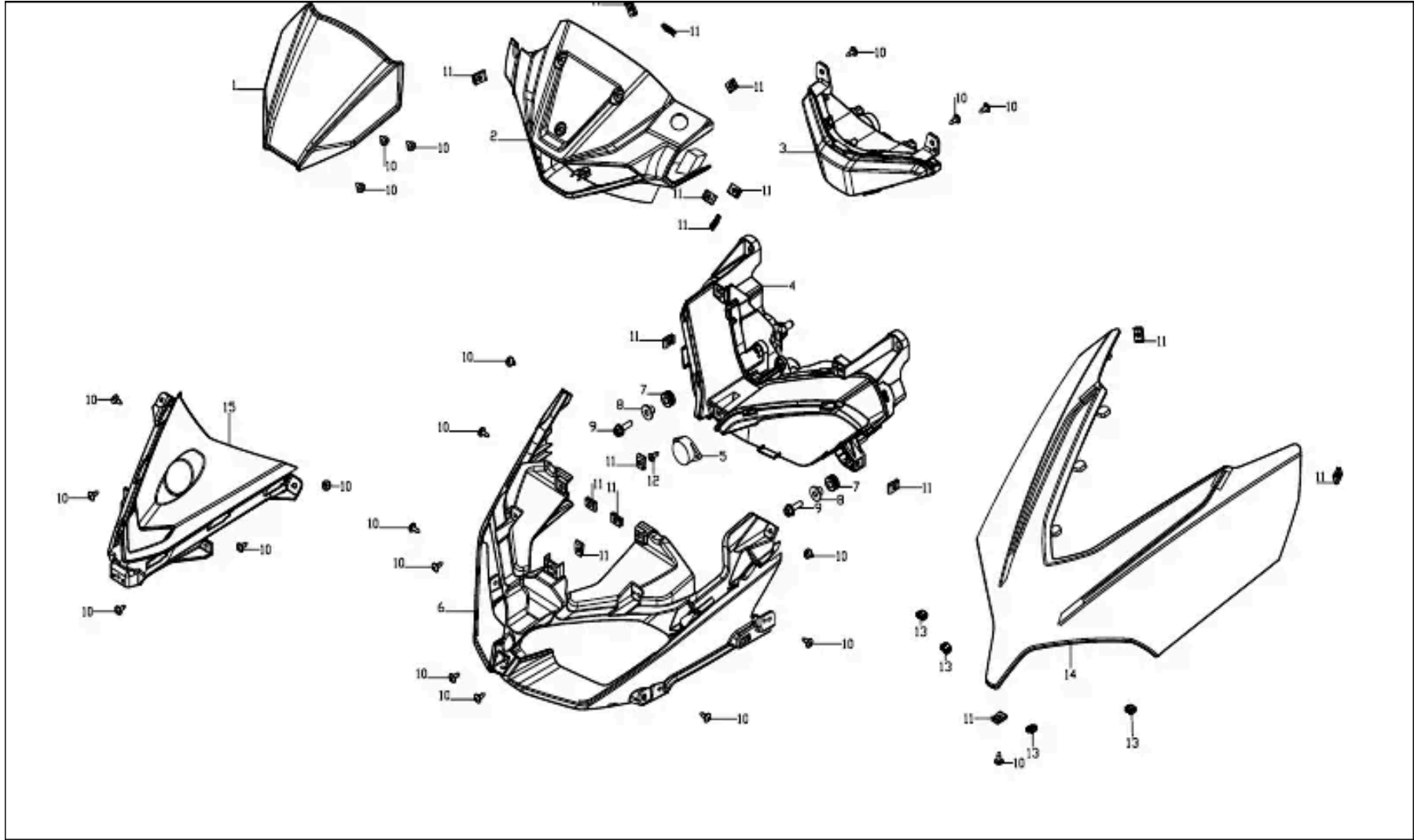
F16 HEADLIGHT ASSY.
