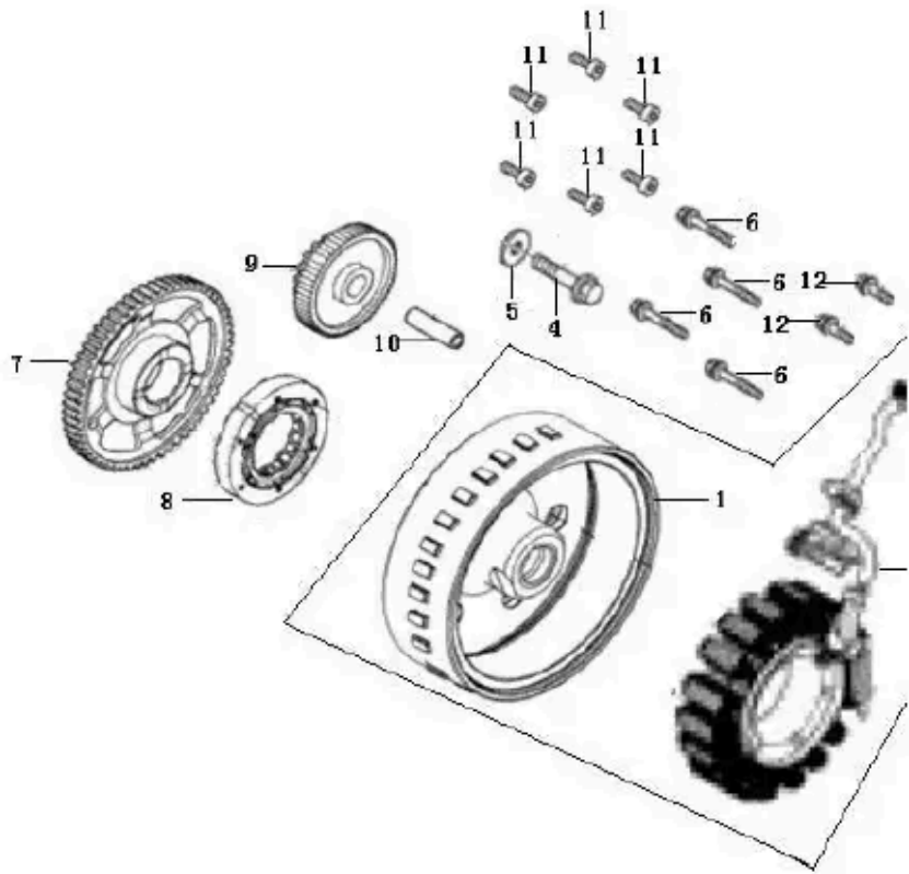
E11 GENERATOR ASSY / ESTATOR COMPLETO
